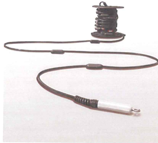
BHC-4 on drum and with spooler device
